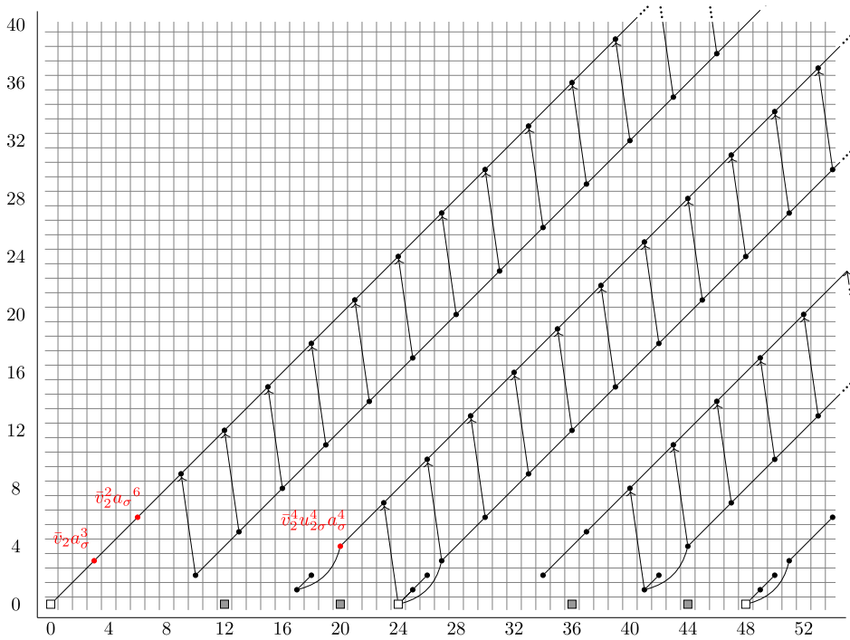
Fig. 4. Important d_7 -differentials and surviving torsion classes in \text{SliceSS}(BP_{\mathbb{R}}) .
