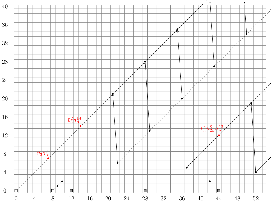
Fig. 5. Important d_{15} -differentials and surviving torsion classes in \text{SliceSS}(BP_{\mathbb{R}}) .
