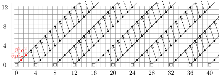
Fig. 3. Important d_3 -differentials and surviving torsion classes in \text{SliceSS}(BP_{\mathbb{R}}) .
