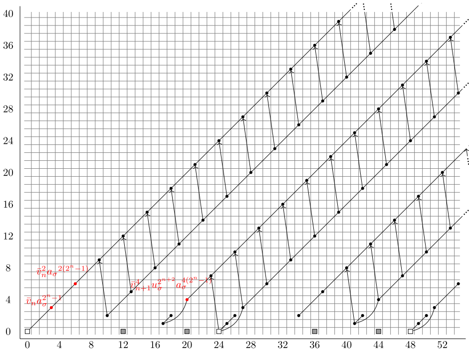
Fig. 6. A part of the slice spectral sequence for BP_{\mathbb{R}} . The classes \bar{v}_n a_{\sigma}^{2^n-1} , \bar{v}_n^2 a_{\sigma}^{2(2^n-1)} , and \bar{v}_{n+1}^4 u_{\sigma}^{2^{n+2}} a_{\sigma}^{4(2^n-1)} survive to the E_{2n+1} -page, hence to the E_{\infty} -page.
