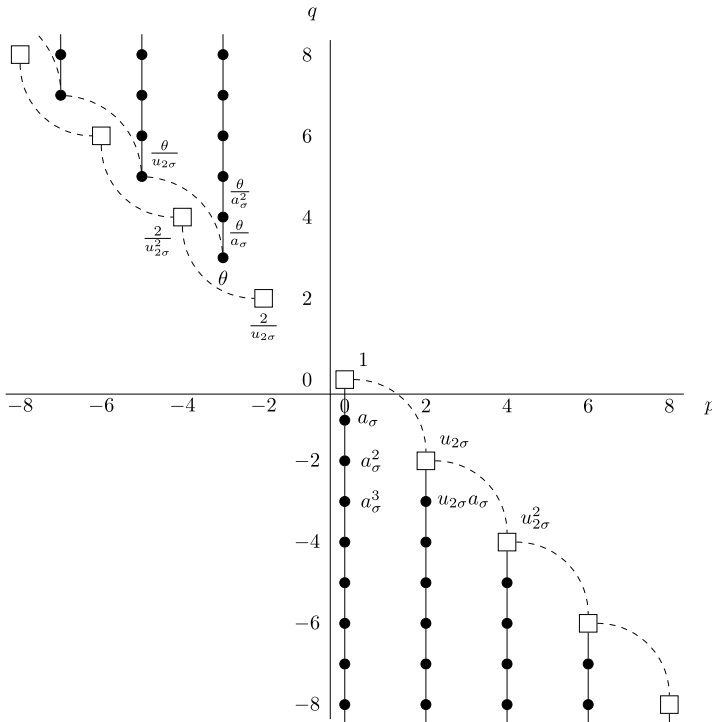
Fig. 2. Coefficient ring of H\mathbb{Z}_{p+q\sigma}^{C_2} . Multiplication by a_\sigma are drawn with solid lines and multiplication by u_{2\sigma} are drawn with dashed lines (not all multiplicative structures are drawn).
