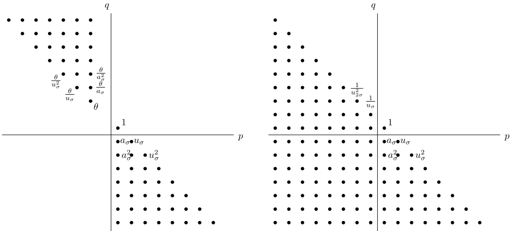
Fig. 1. The coefficient rings of H\mathbb{F}_2_{p+q\sigma} (left) and F(EC_{2+}, H\mathbb{F}_2)_{p+q\sigma} (right). The map H\mathbb{F}_2_{p+q\sigma} \rightarrow F(EC_{2+}, H\mathbb{F}_2)_{p+q\sigma} induces an isomorphism in the range p \geq 0 .
