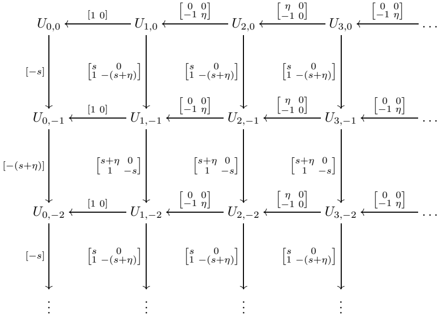
FIGURE 1. The bicomplex (U_{*,*}, \partial^h, \partial^v) for \Gamma = k[s]/(s^2 = \eta s)
