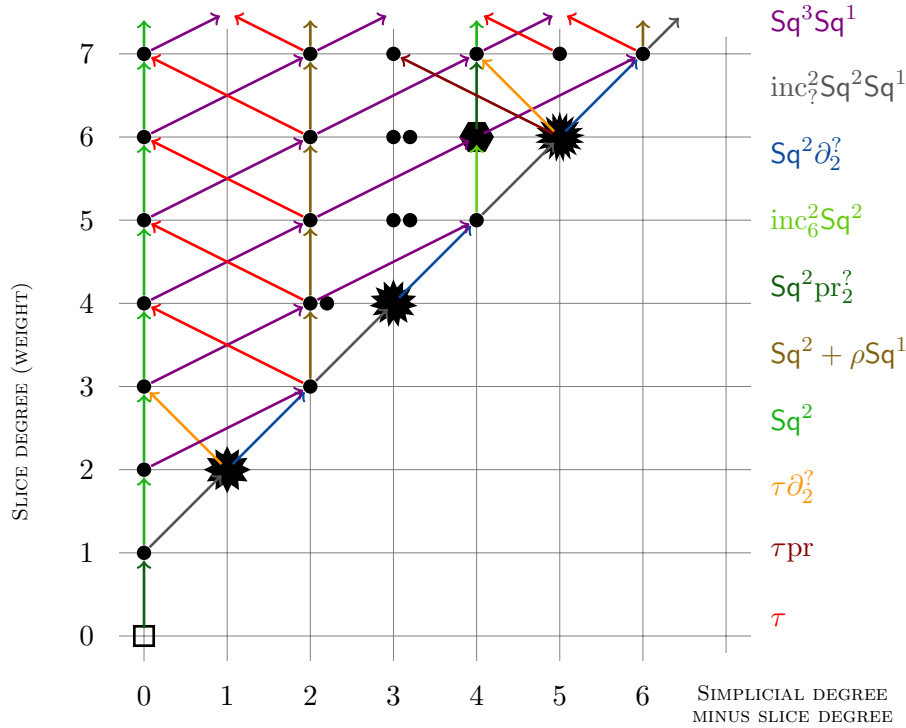
Figure 4.1. The first slice differential for \mathbf{1}_\Lambda .
