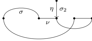
FIGURE 3. Steenrod module structure of the 20-skeleton of B ; the bottom cell (in dimension 0) is on the left; straight lines are \text{Sq}^4 , and curved lines correspond to \text{Sq}^8 and \text{Sq}^{16} , in order of increasing length. The bottom two attaching maps of B are labeled. The map \sigma_2 is shown.
