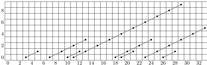
Figure 2. The homotopy of \overline{\mathrm{THH}}(ku; k(1)) .
