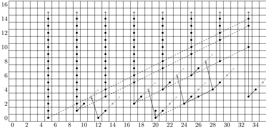
Figure 8. The \eta -Bockstein E_2 -page.
