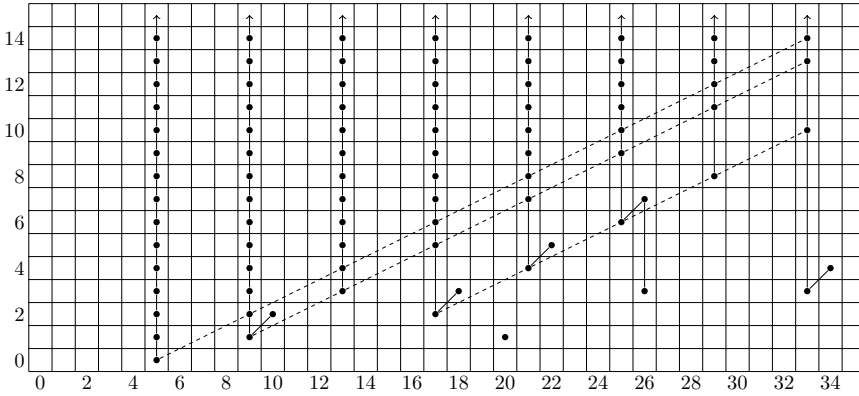
Figure 5. \overline{\text{THH}}_*(ko) through degree 34.
