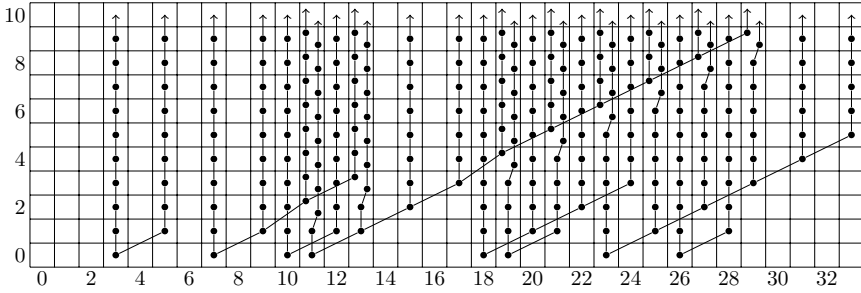
Figure 3. The v_0 -Bockstein spectral sequence converging to \overline{\text{THH}}_*(ku) .
