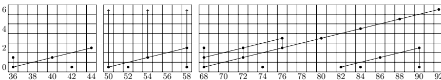
Figure 6. The torsion between degrees 36 and 92.
